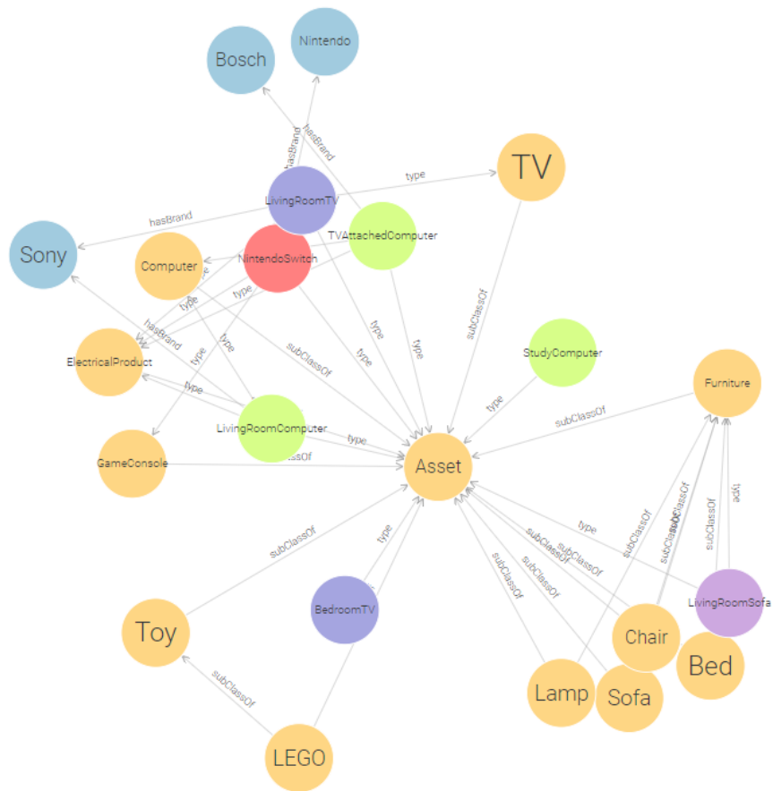
FIGURE 14.4: An example of an RDF model in GraphDB that describes house assets. This is only a demonstration graph and the information inside is artificial and not true.
