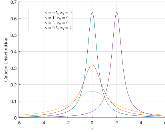
FIGURE 2.4: Cauchy Distribution.
